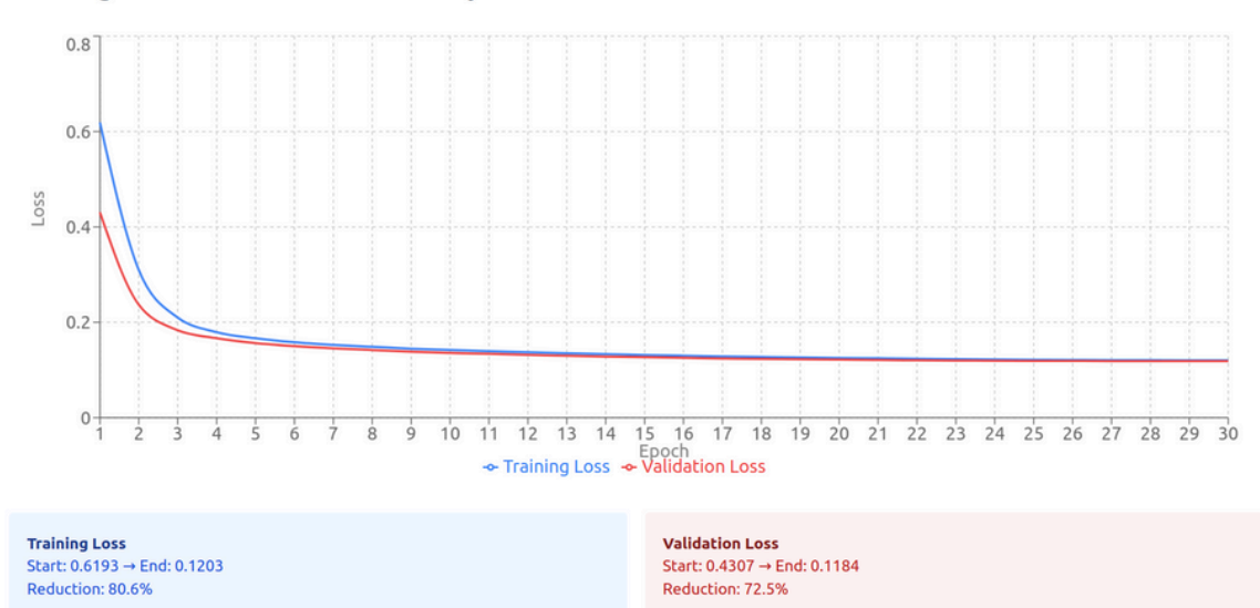
Training and Validation Loss Over Epochs
