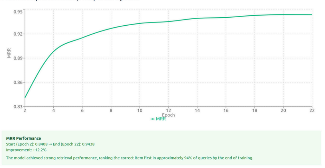
Mean Reciprocal Rank (MRR) Over Epochs
